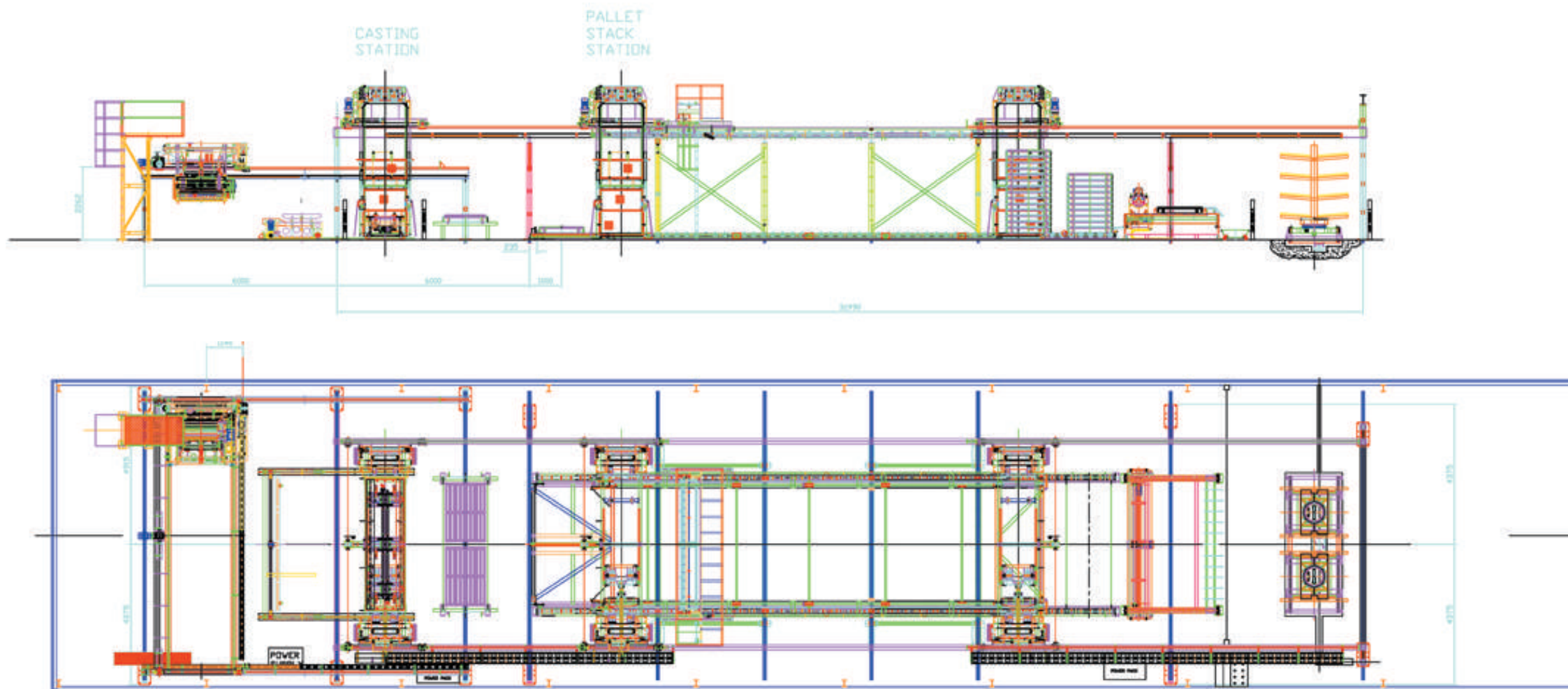
Automatic Dry Cast System
