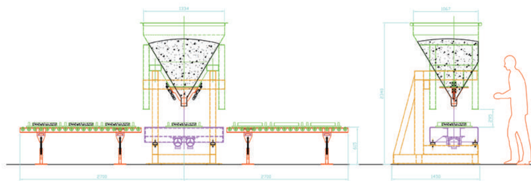
Wetcast Dosing System
